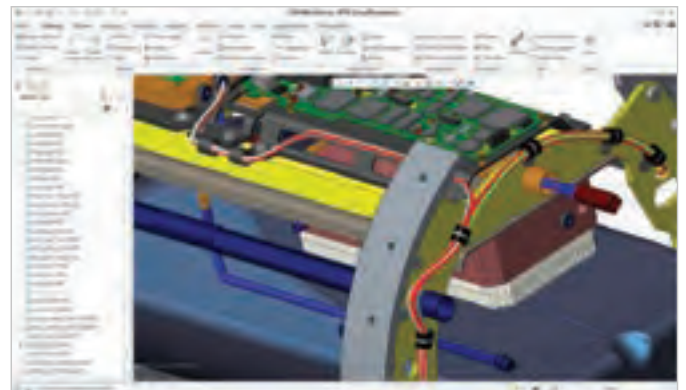
Automated cabling design capabilities make it easy to move components and connectors without manually rerouting wires and cables.
